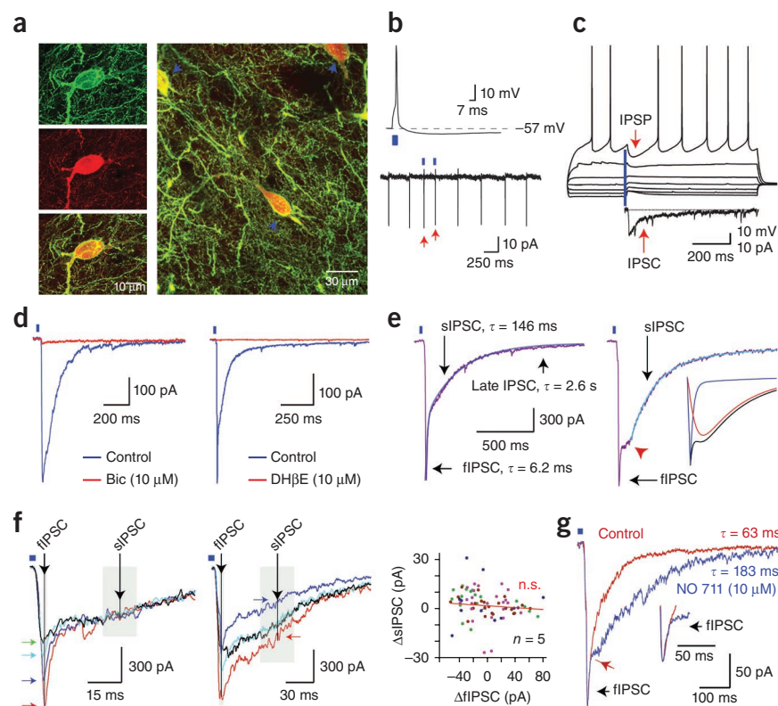
Figure 1 Characterization of GABAergic IPSCs elicited in SPNs with optogenetic stimulation of ChAT interneurons. (a) Confocal images of a ChR2-YFP-expressing neuron (top left) immunostained for ChAT (middle; bottom, overlay). A larger field is shown at the right. (b) Top, optically elicited action potential in a ChAT interneuron. Bottom, a cell-attached recording of spontaneous activity and optically evoked action potentials (red arrows) of a ChAT interneuron. (c) Optogenetically elicited IPSPs in an SPN (arrow) efficiently blocked firing induced by current injection. Bottom trace, corresponding IPSC ( V_{\text{hold}} = -80 mV). (d) Optogenetically elicited IPSCs in two SPNs (blue traces) were blocked by bicuculline (Bic, left) or DH \beta E (right, red traces). (e) Kinetic components of the compound IPSC. Left, three distinct components of the IPSC exhibiting different \tau_{\text{decay}} values. Right, non-monotonic transition between the fIPSC and the sIPSC. Note the negative inflection following the transition (red arrowhead). Inset, decomposition of the compound IPSC (black trace) into a fIPSC (blue trace) and sIPSC (red trace). (f) Independent trial-to-trial amplitude variance of the fIPSC and the sIPSC. Left, overlay of four responses exhibiting identical sIPSC, but different fIPSC, components (colored arrows point to fIPSC peaks). Shaded areas are averaging windows. Middle, variable sIPSC components. Right, relative sIPSC amplitudes plotted against corresponding relative peak fIPSC amplitudes ( n = 5 ). Red line is linear regression (n.s., not significant, P > 0.2 ). (g) Inhibition of GAT-1 selectively prolonged the sIPSC. Note that the fIPSC was unaffected (arrow and inset). Red arrow, transition point of the response components. In all figures, the blue bars represent optical stimuli.
